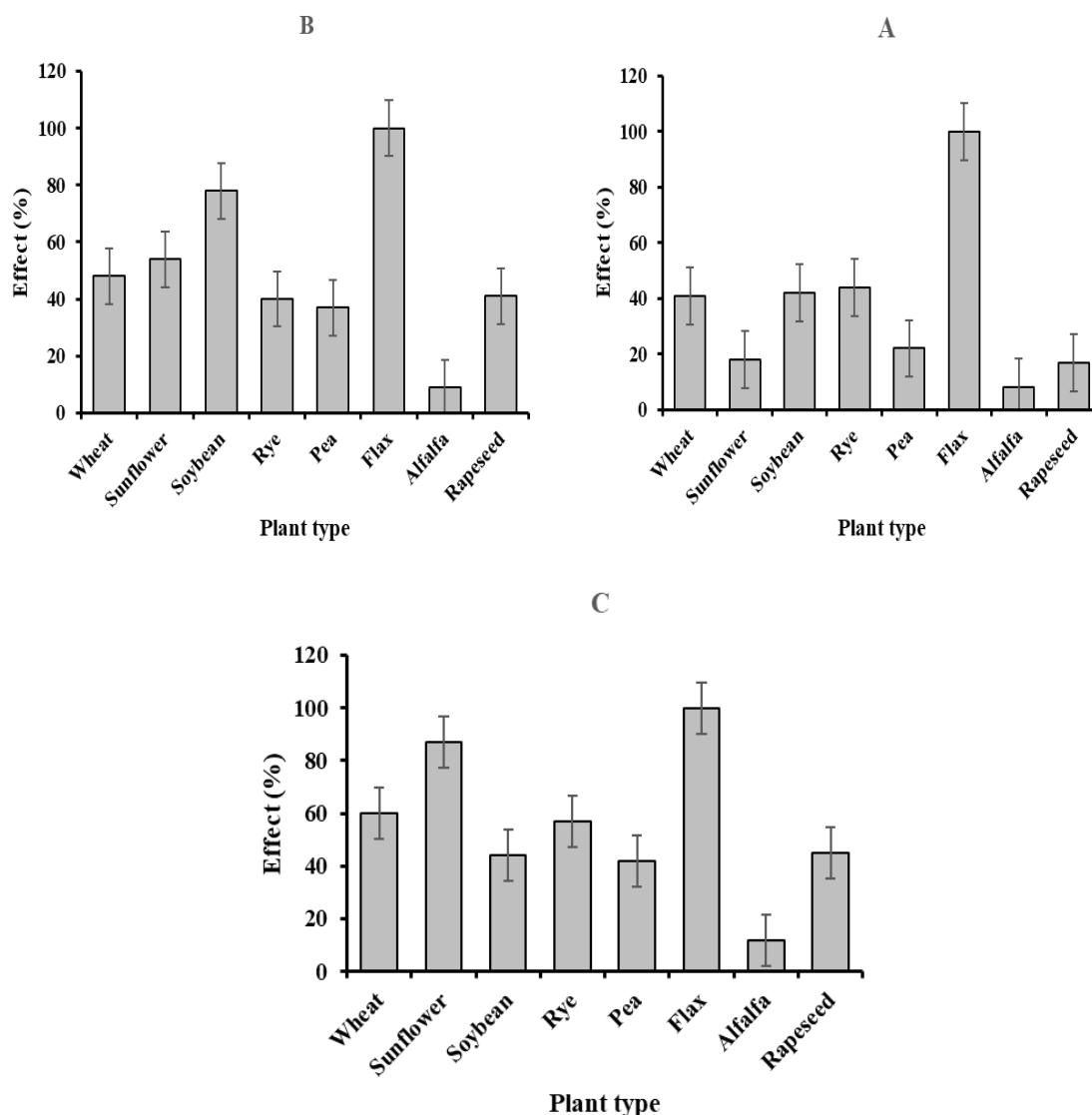
Fig. 1: The percentage effect of proposed plants for the crop rotation with lentil on human health (A), ecosystems (B) and resources (C) Comparing processes; Method: ReCiPe 2016 Endpoint (E) v1.03/Damage assessment
