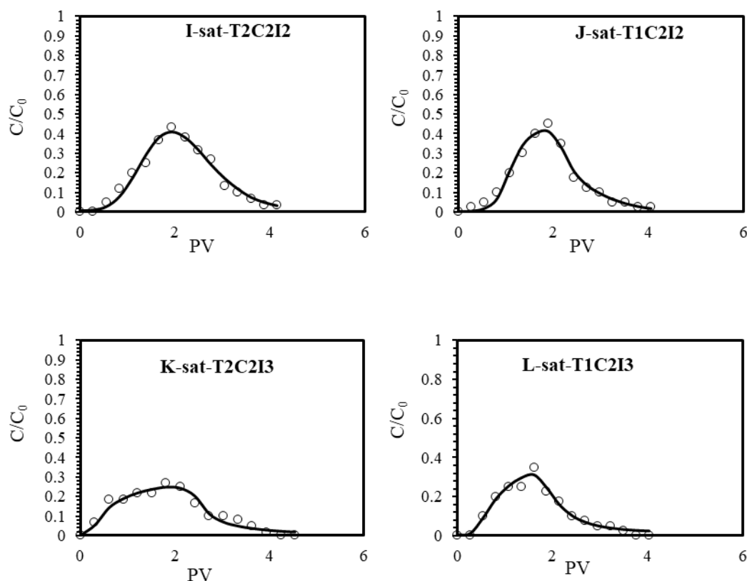
Fig. 6. Chloride breakthrough curves under saturated conditions. T1 and T2 represent conventional (moldboard plow) and minimum (chisel) tillage, respectively. C1 and C2 denote the cover crop Lathyrus sativus (grass pea) and the control treatment, respectively. I1, I2, and I3 correspond to 50% intercropping, sole summer squash cultivation, and sole green bean cultivation, respectively
