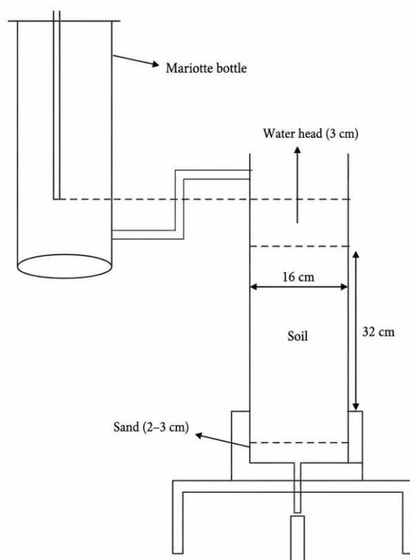
Fig. 2. Schematic of saturated hydraulic conductivity measurement
