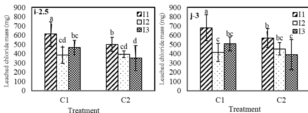
Fig. 5. Comparison of the effect of cropping pattern on the mass of chloride in the effluent Aat different pore volumes (PV): (a) 1, (b) 1.5, (c) 2, and (d) 3.5. Comparison of the two-way interaction effect of tillage \times cover crop on chloride mass in the effluent (mg) at PV: (e) 0.5, (f) 1, (g) 1.5, and (h) 2. Comparison of the two-way interaction effect of cover crop \times cropping pattern on chloride mass in the effluent (mg) at PV: (i) 2.5 and (j) 3. Treatments T1 and T2 represent conventional (moldboard plow) and minimum (chisel) tillage, respectively. Likewise, C1 and C2 correspond to the cover crop Lathyrus sativus (grass pea) and the control treatment, respectively, while I1, I2, and I3 denote 50% intercropping, sole summer squash cultivation, and sole green bean cultivation, respectively. Columns sharing the same letter are not significantly different at the 5% probability level according to Duncan's multiple range test. Furthermore, vertical bars on each column indicate data variability expressed as standard deviation
